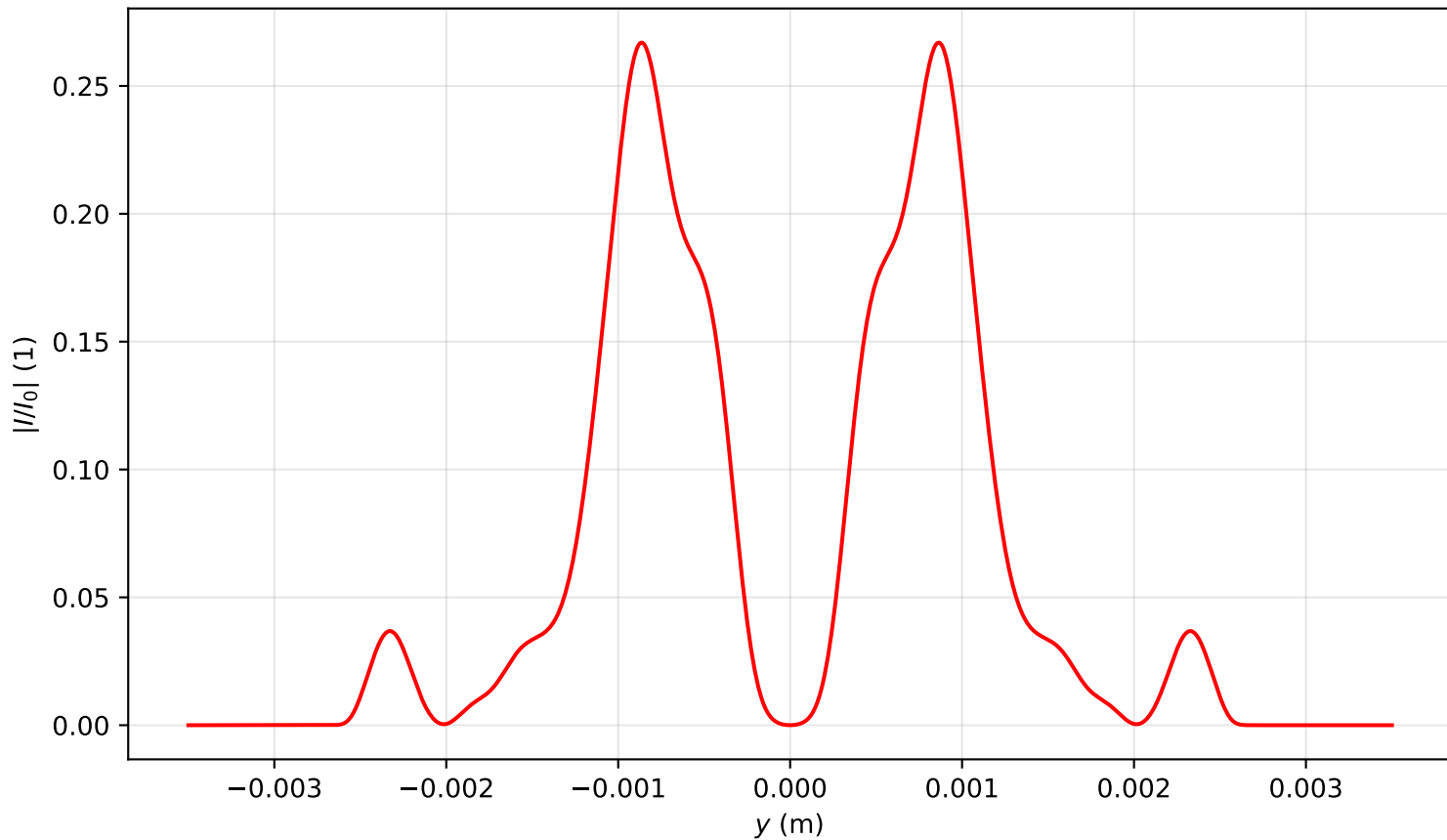
Intensity profile I(x=0, y, z=3.901)/I_0 , P_{in}=6.0P_{cr} , artificial time
